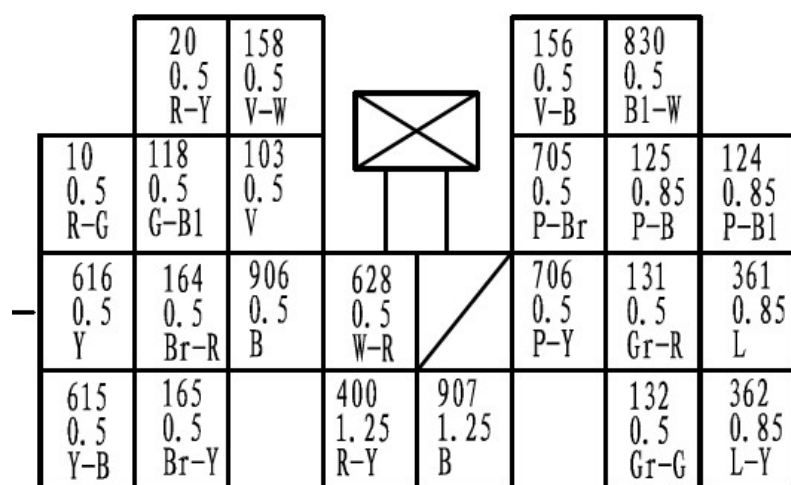
(1)接仪表板线束
